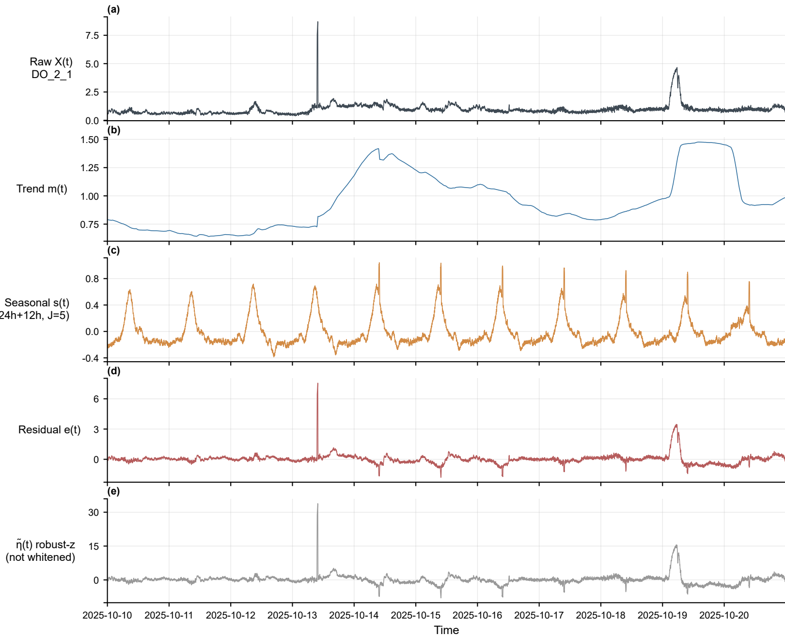
Multi-scale decomposition — DO_2_1 (aerobic, min) [2025-10-10~2025-10-20]
